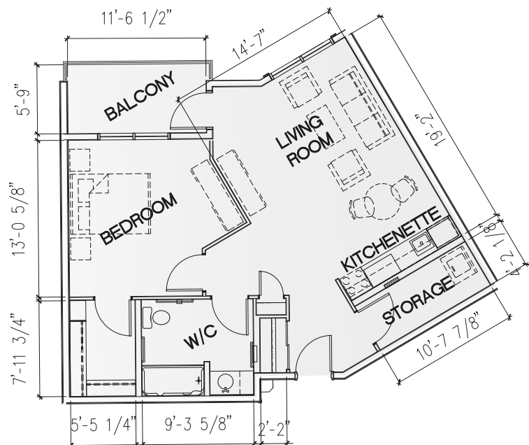
C One bedroom unit 760 sq ft
