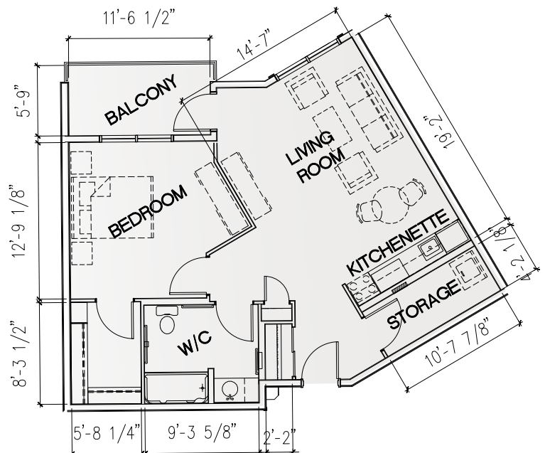
C One bedroom unit 760 sq ft
